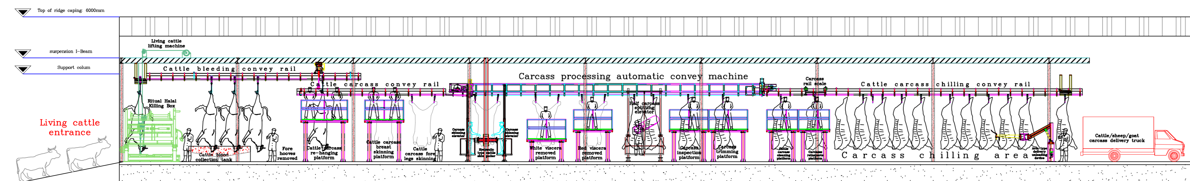
The 50-100cattle per day abattoir elevation layout
