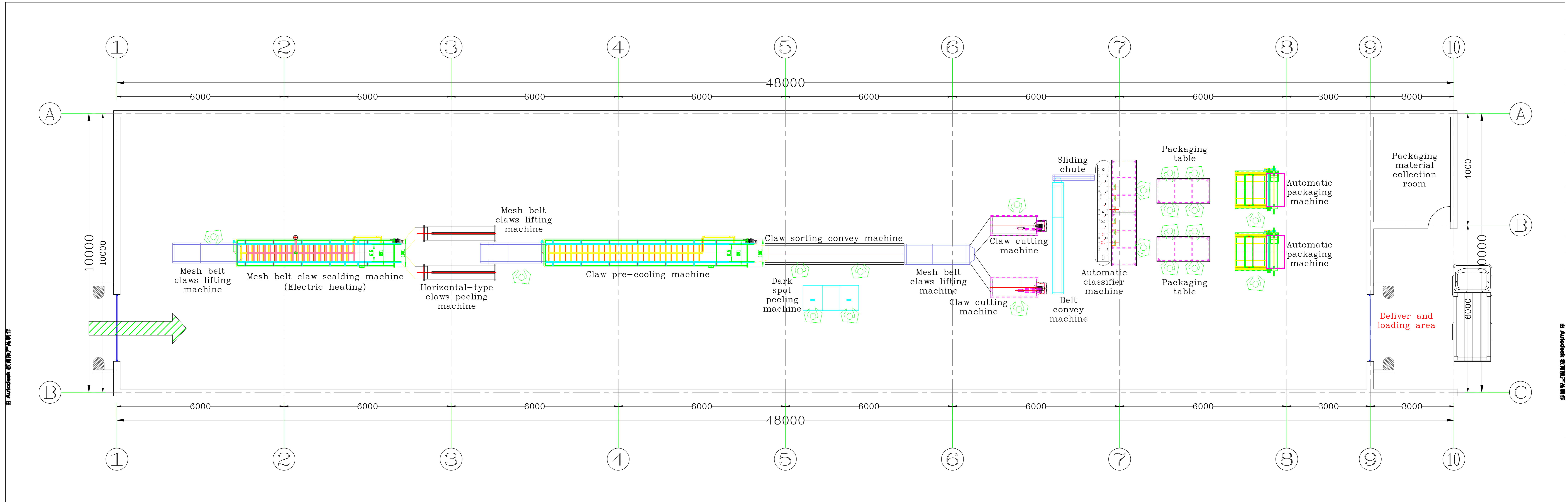
The 2Tons per hour chicken claws peeling systems floor plan layout
