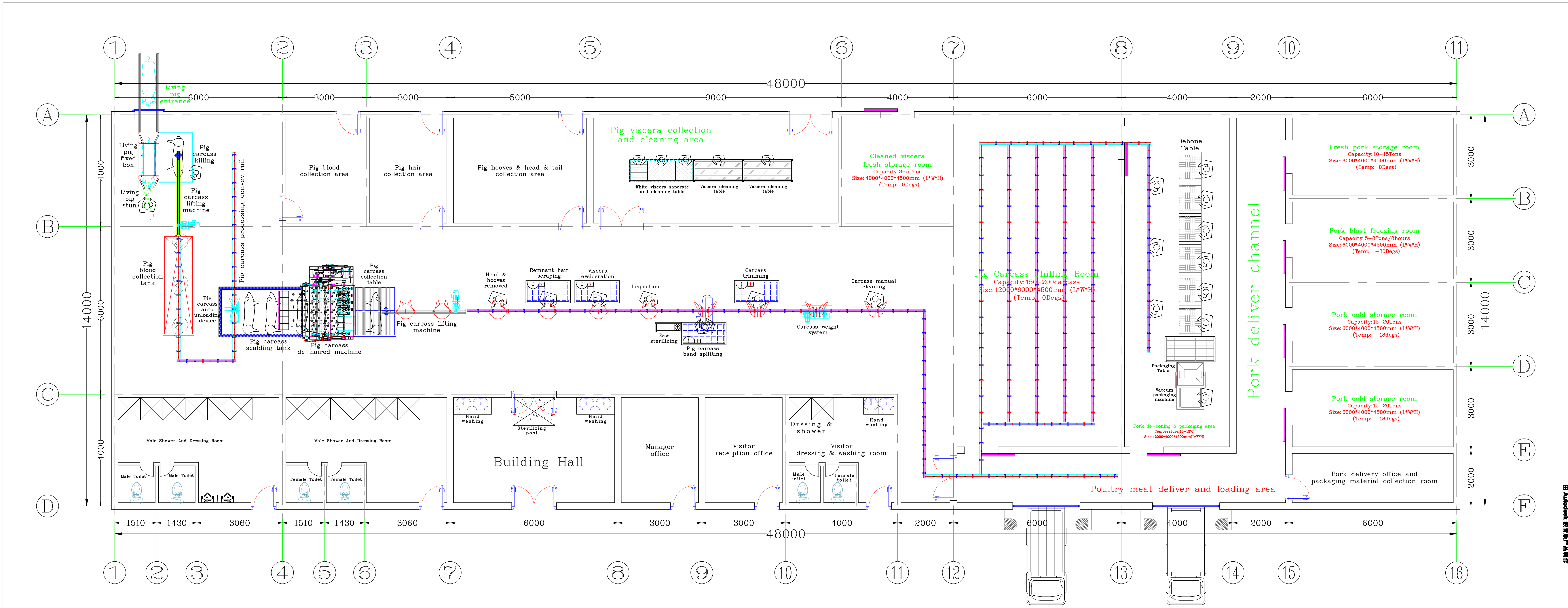
The 200pig per shift abattoir floor plan layout
