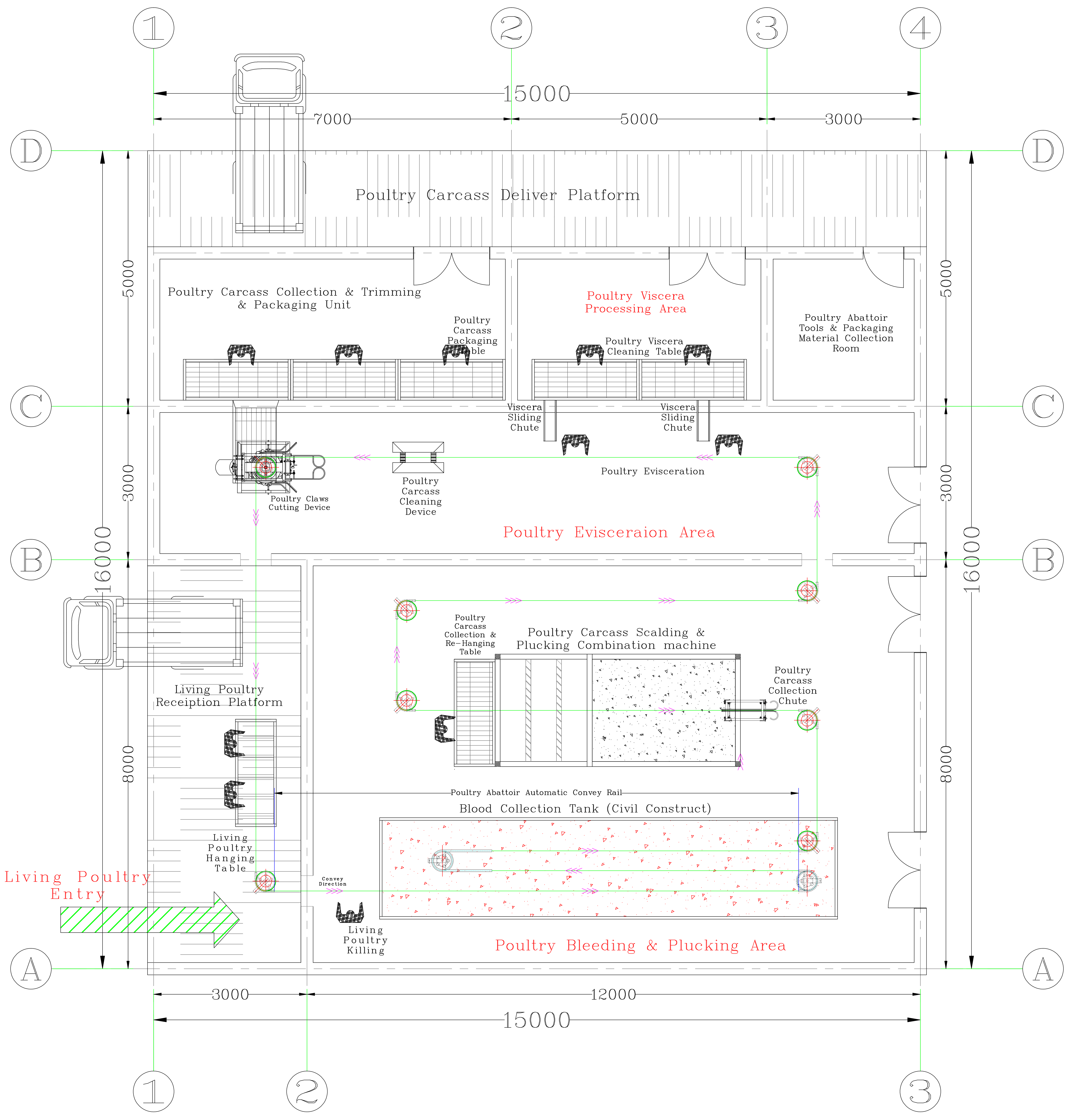
The 300-500Poultry/Broiler Per Hour Abattoir Design Layout
