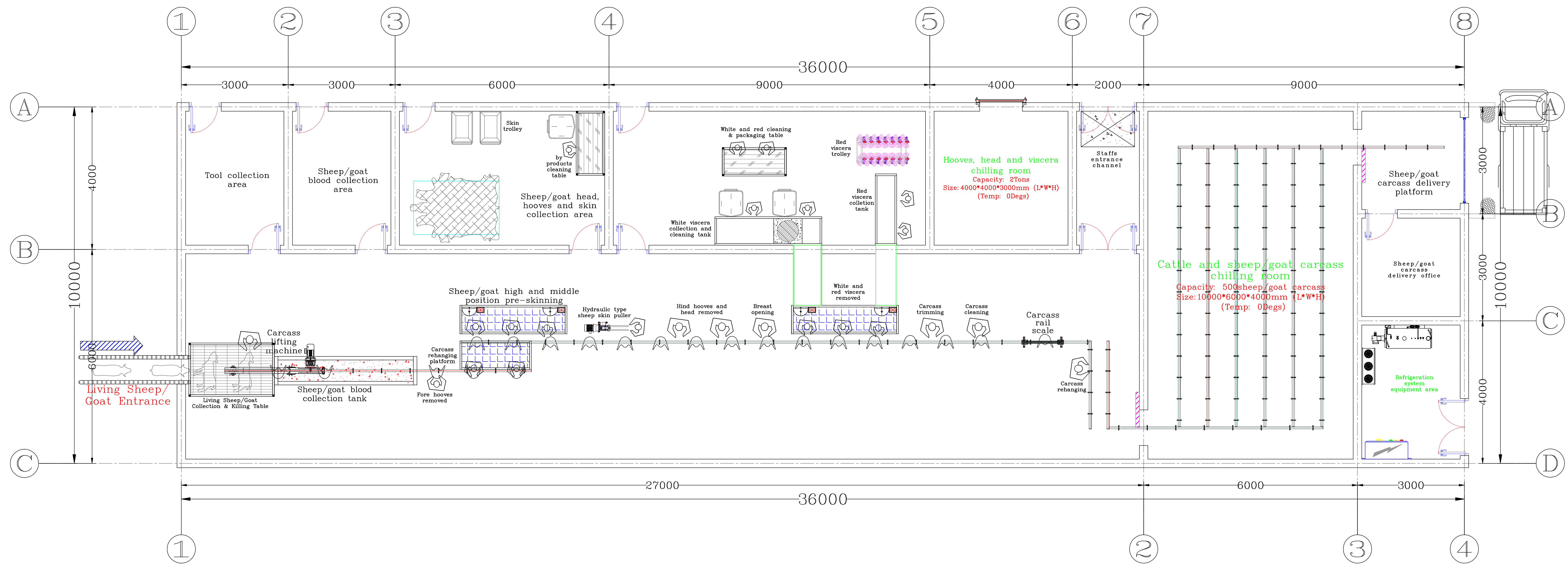
The 500sheep/goat per day abattoir floor plan layout
