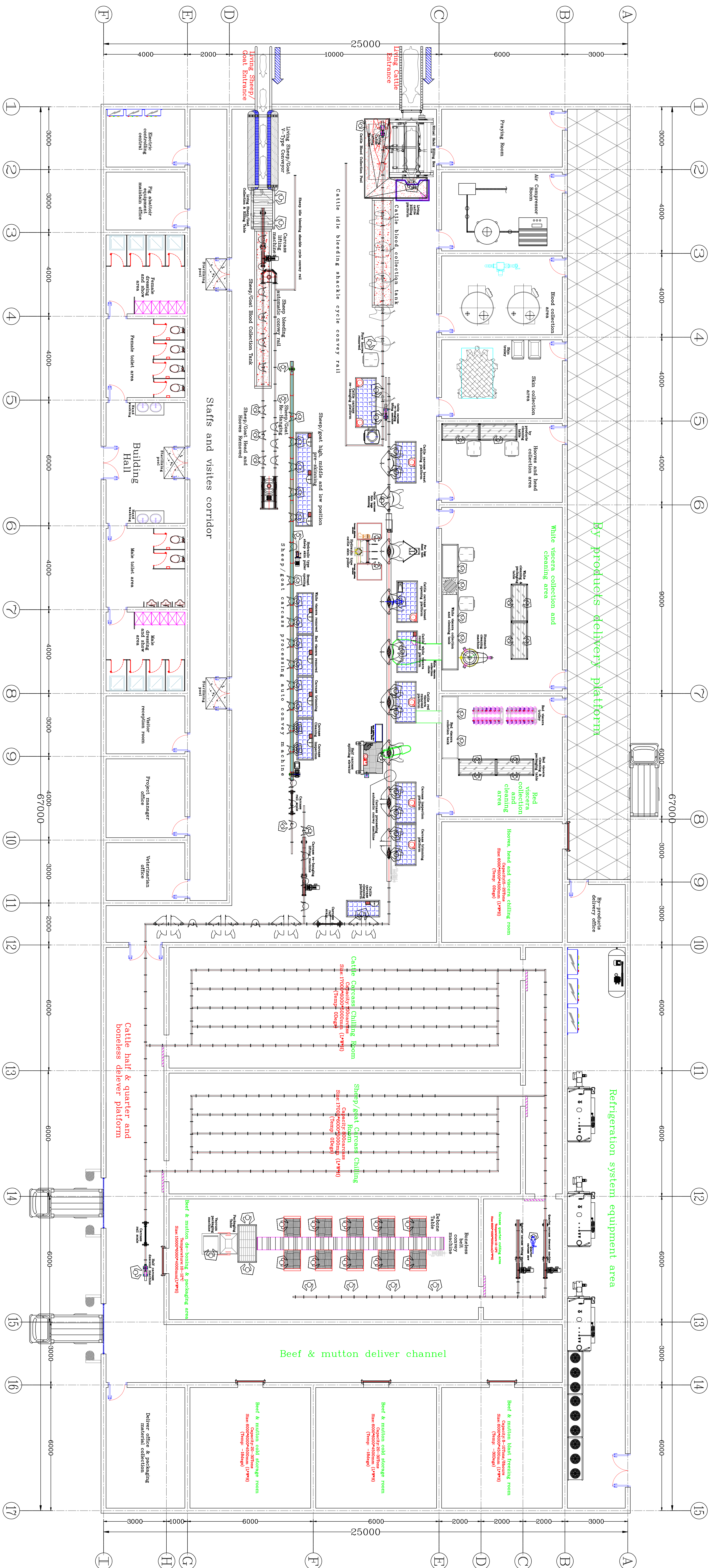
The 100cattle and 800sheep/goat per day abattoir floor plan layout
